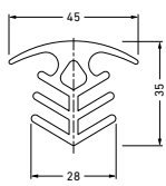
FA 15/4535 Material: PVC Joint width max.: 20 mm
